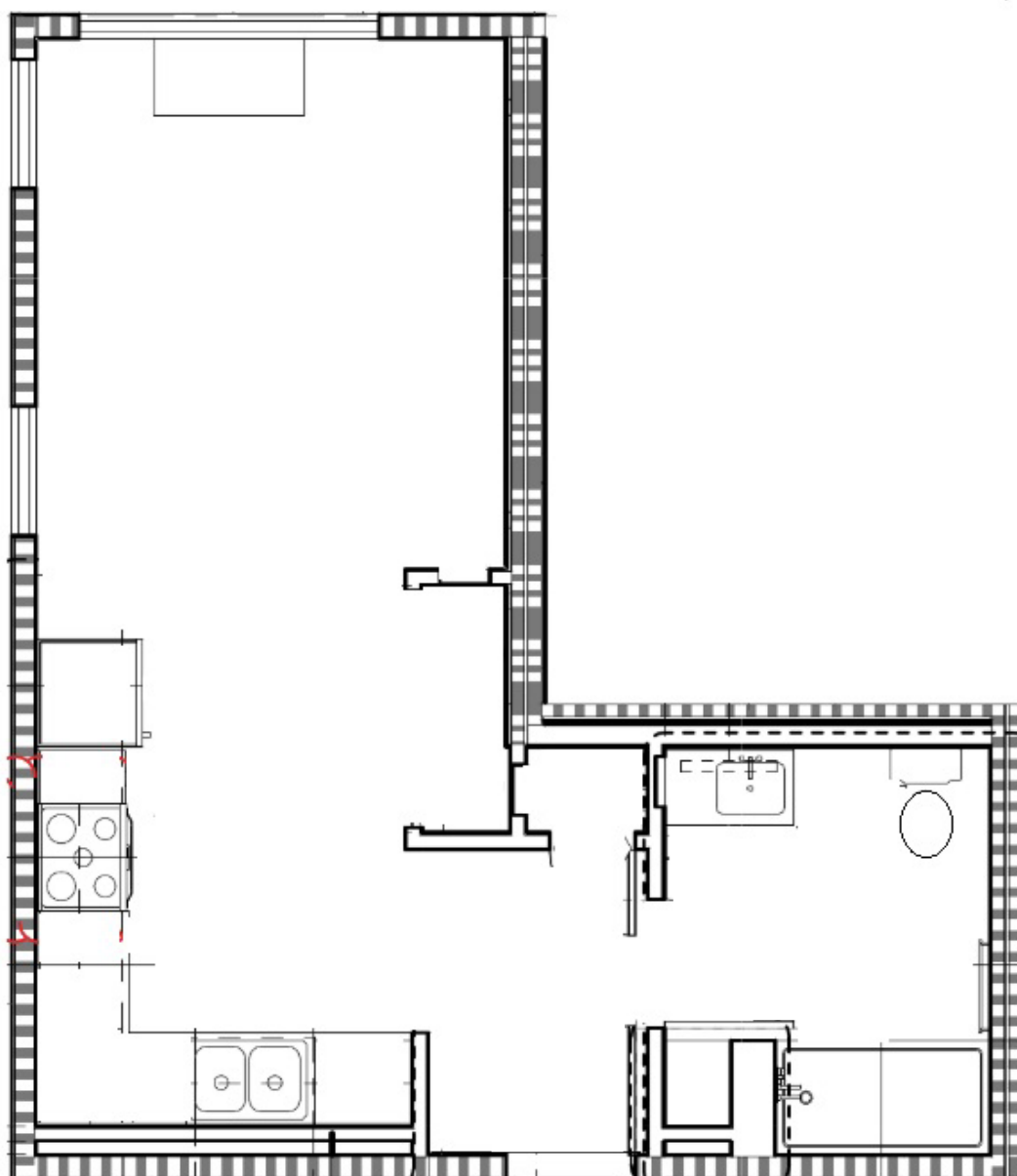
Studio Unit Type C - 400 Sq FT
