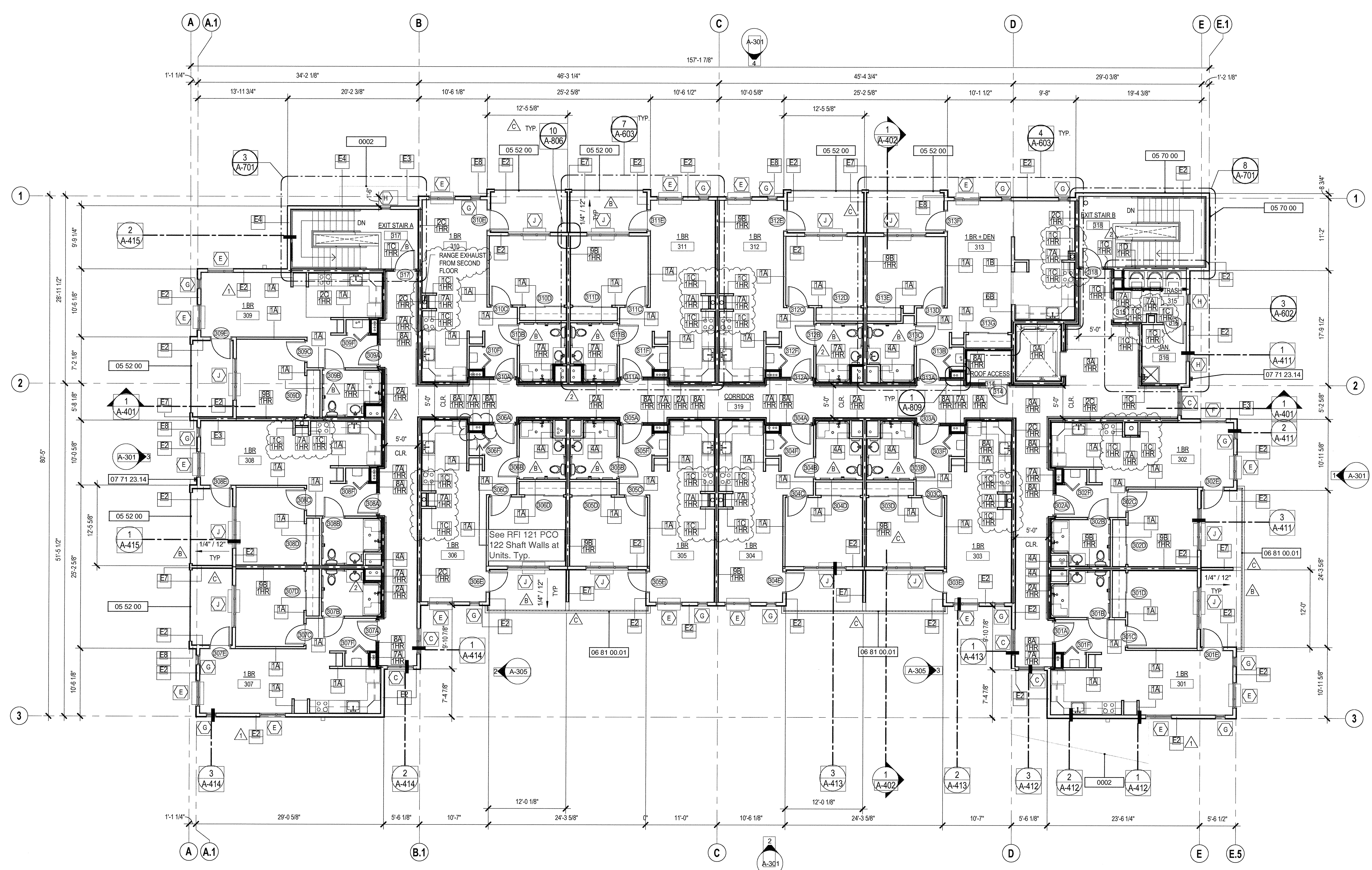
THIRD FLOOR PLAN 1/8" = 1'-0"
