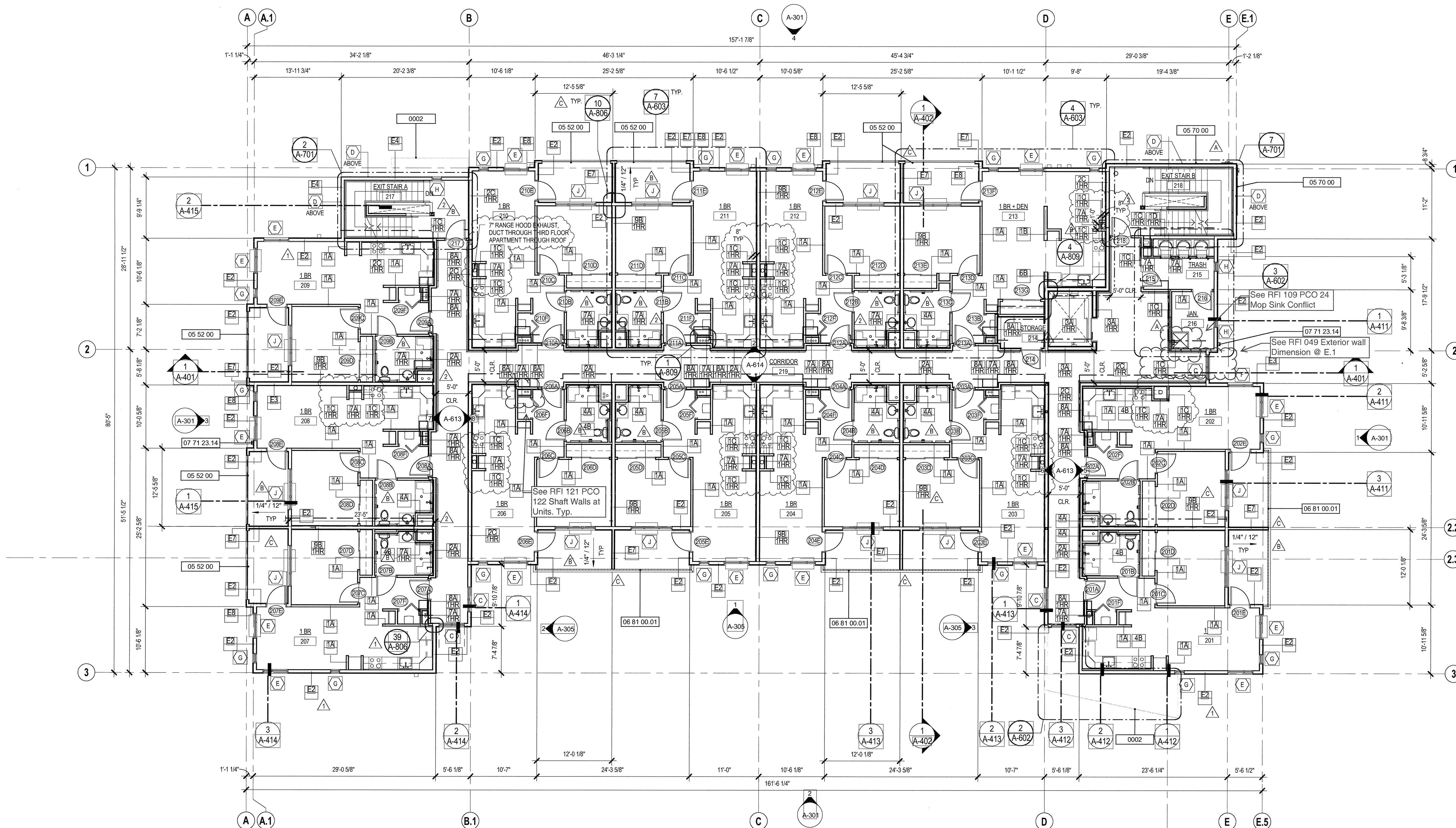
SECOND FLOOR PLAN 1/8" = 1'-0"
