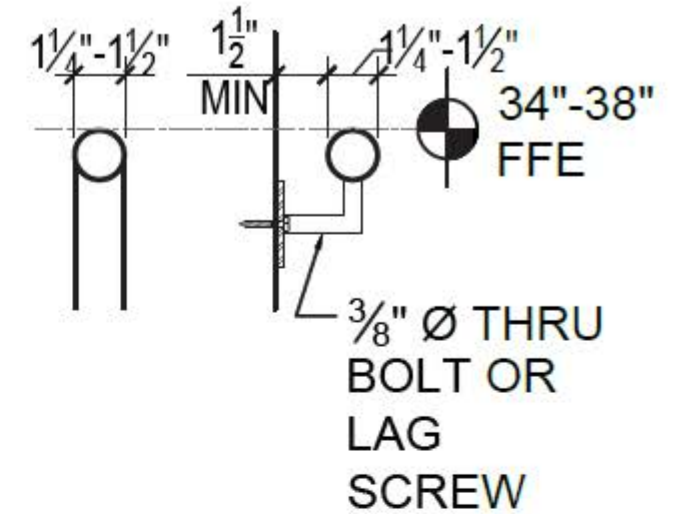
HANDRAIL SECTION
