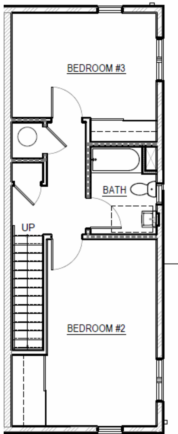
Second Floor
